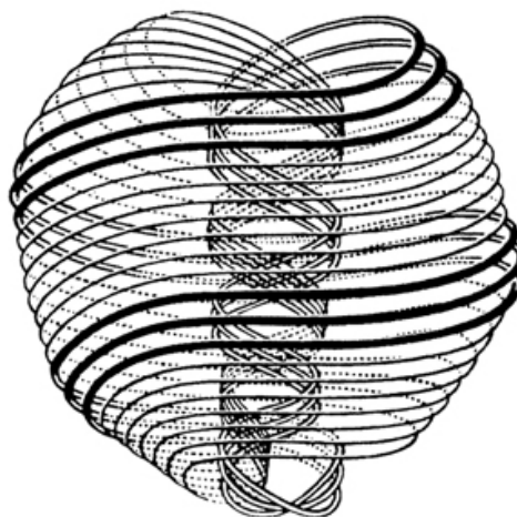
Figure 1 – Subatomic particle
